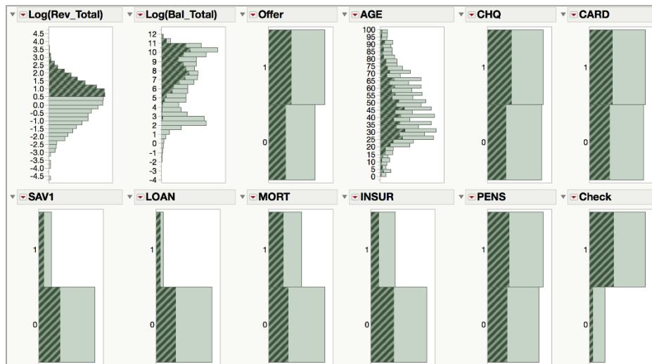
Exhibit 4 Relationships between Transformed Variables and Other Variables
