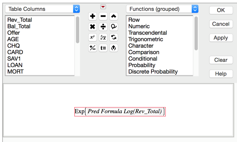
Exhibit 16 Transforming Predicted \text{Log}(\text{Rev\_Total}) to Predicted \text{Rev\_Total}
