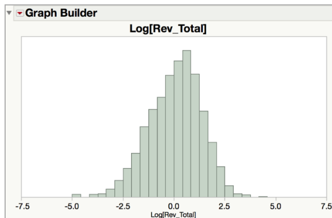
Exhibit 2 Transformed Total Revenue Using Log Transformation
