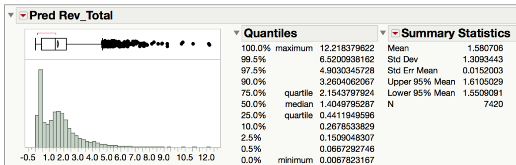
Exhibit 17 Distribution of Predicted \text{Rev\_Total}
