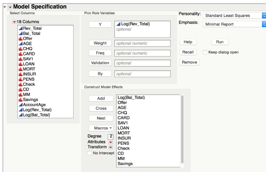
Exhibit 5 Fit Model Dialog
